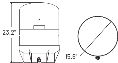
60L (10-gallon) hydropneumatic tank
